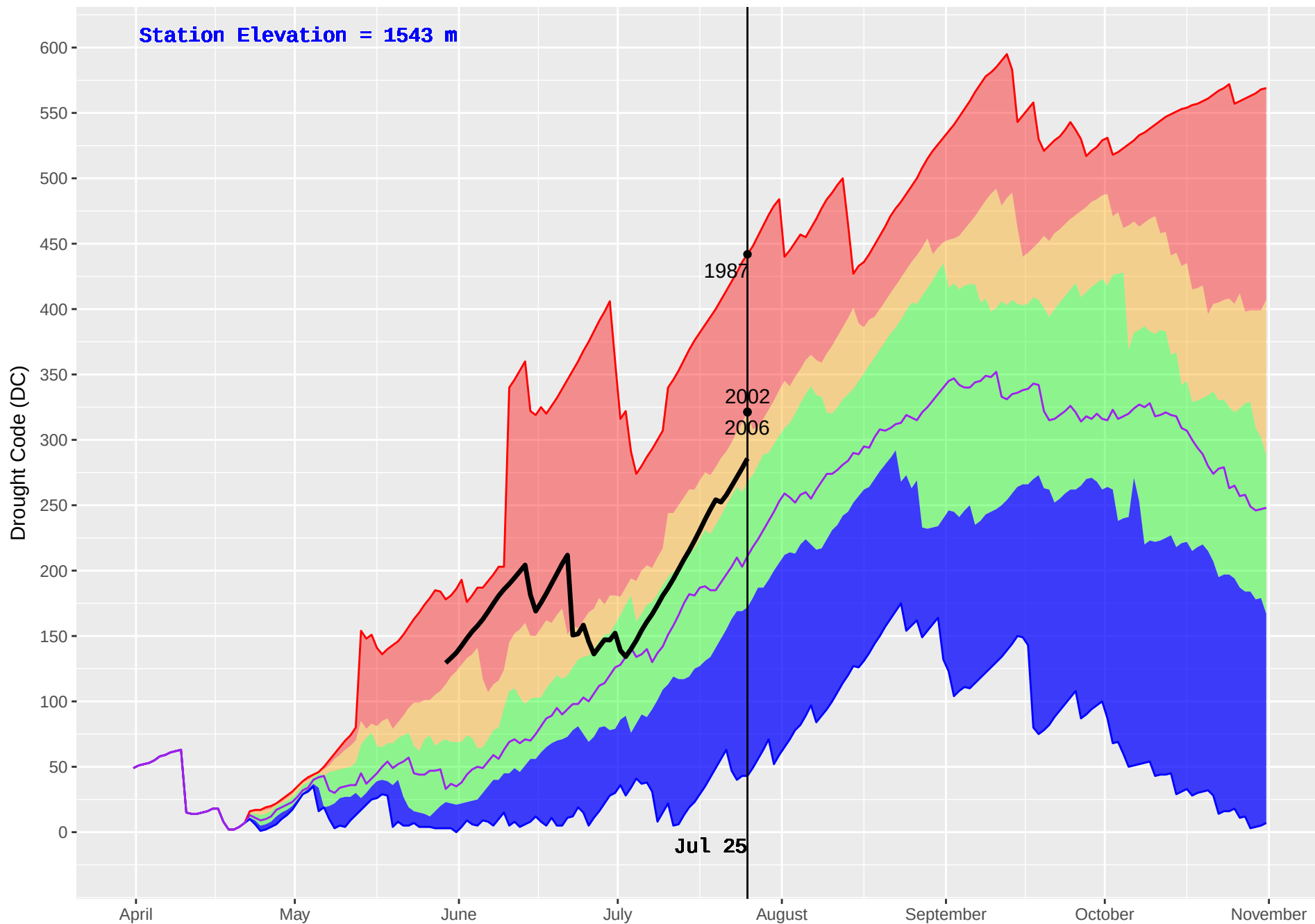
CAHILTY (253) : Historical (1987–2016) and Current (2018) Noon Drought Code (DC)
