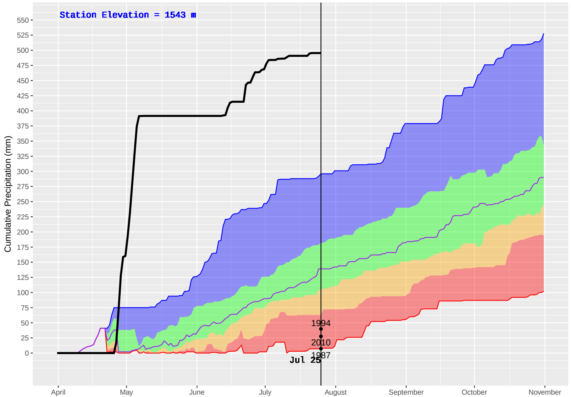
CAHILTY (253) : Historical (1987–2016) and Current (2018) Noon Cumulative Precipitation
