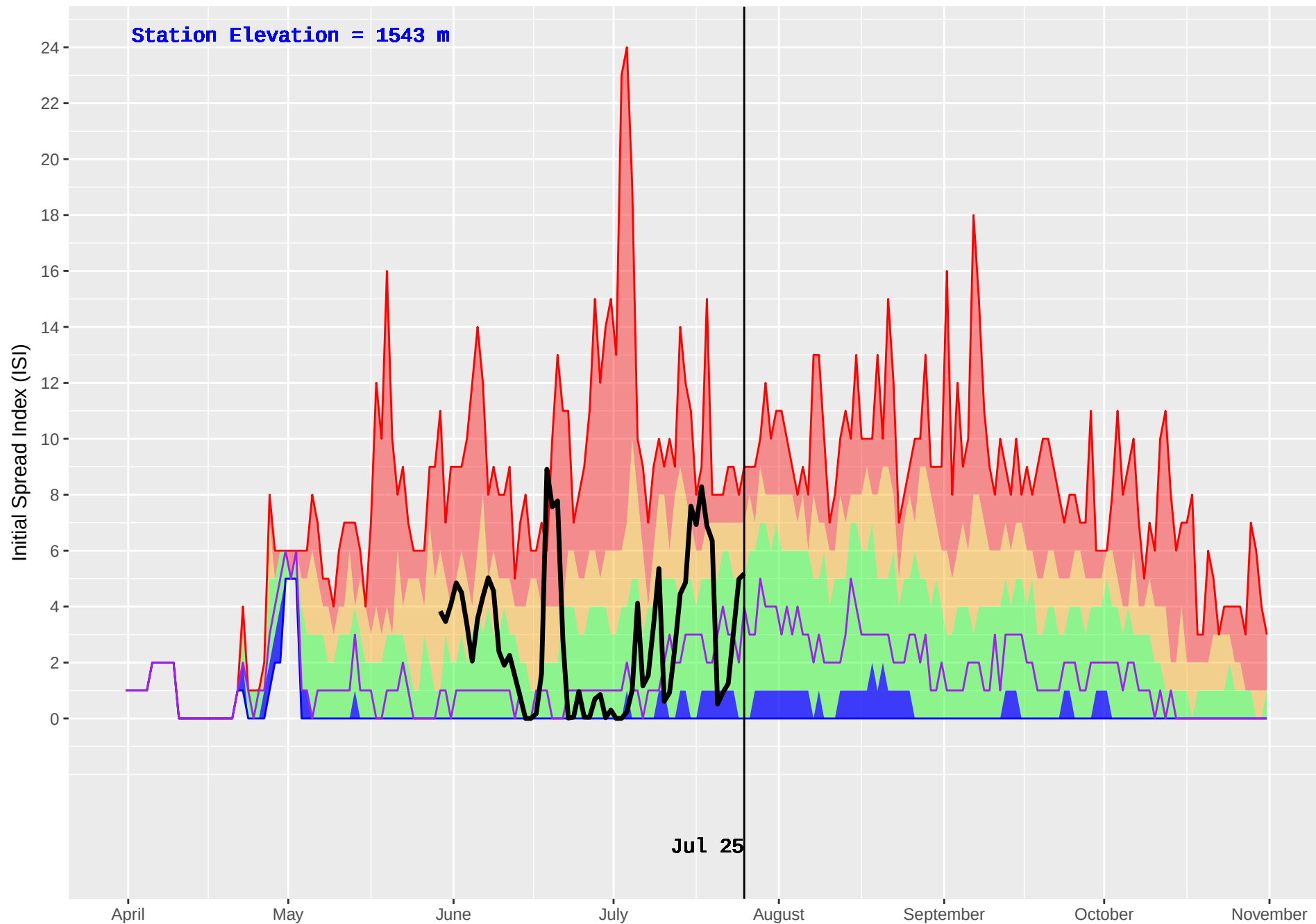
CAHILTY (253) : Historical (1987–2016) and Current (2018) Noon Initial Spread Index (ISI)
